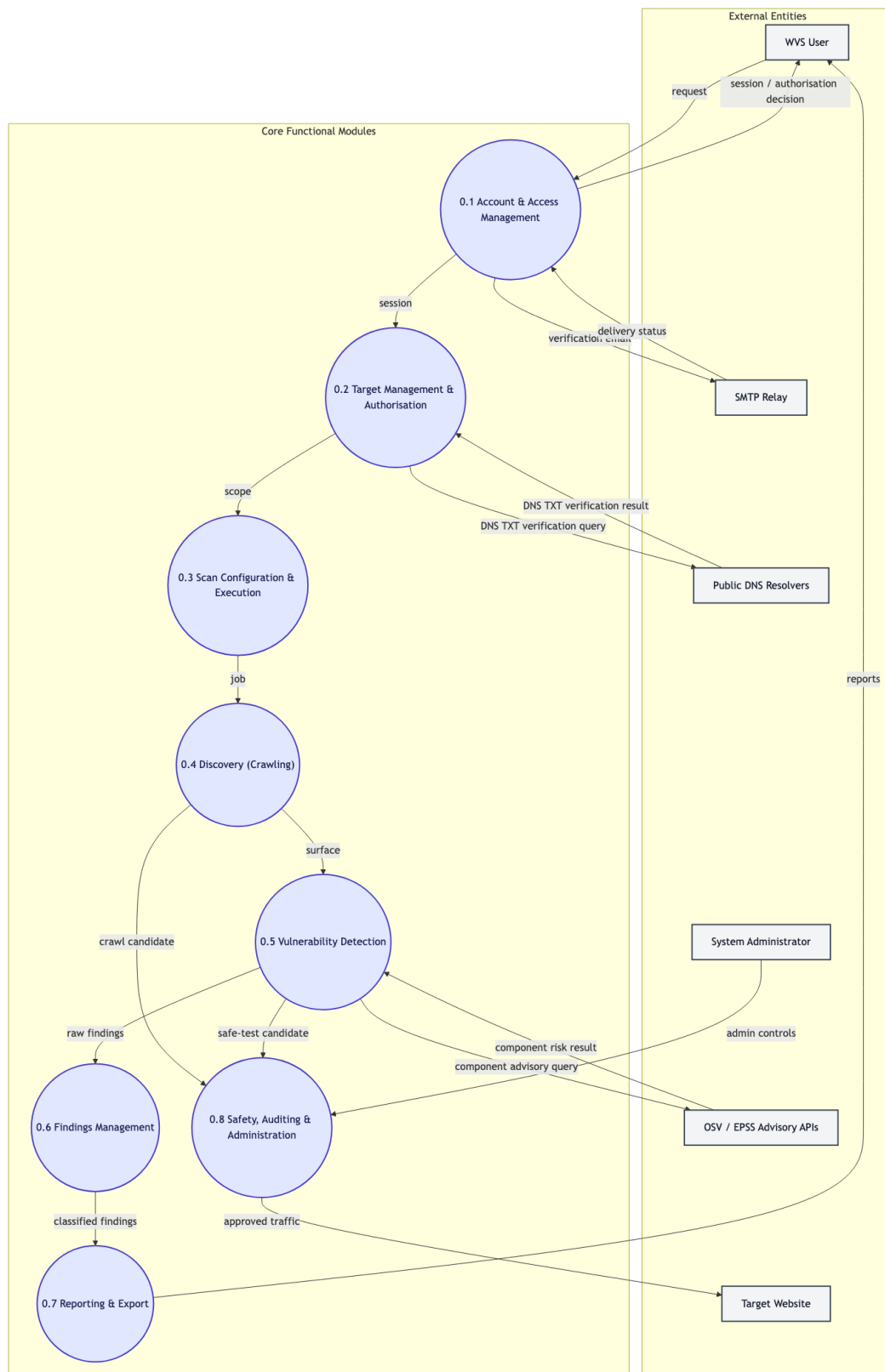
Figure 2: Level 1 DFD with 8 functional groups
