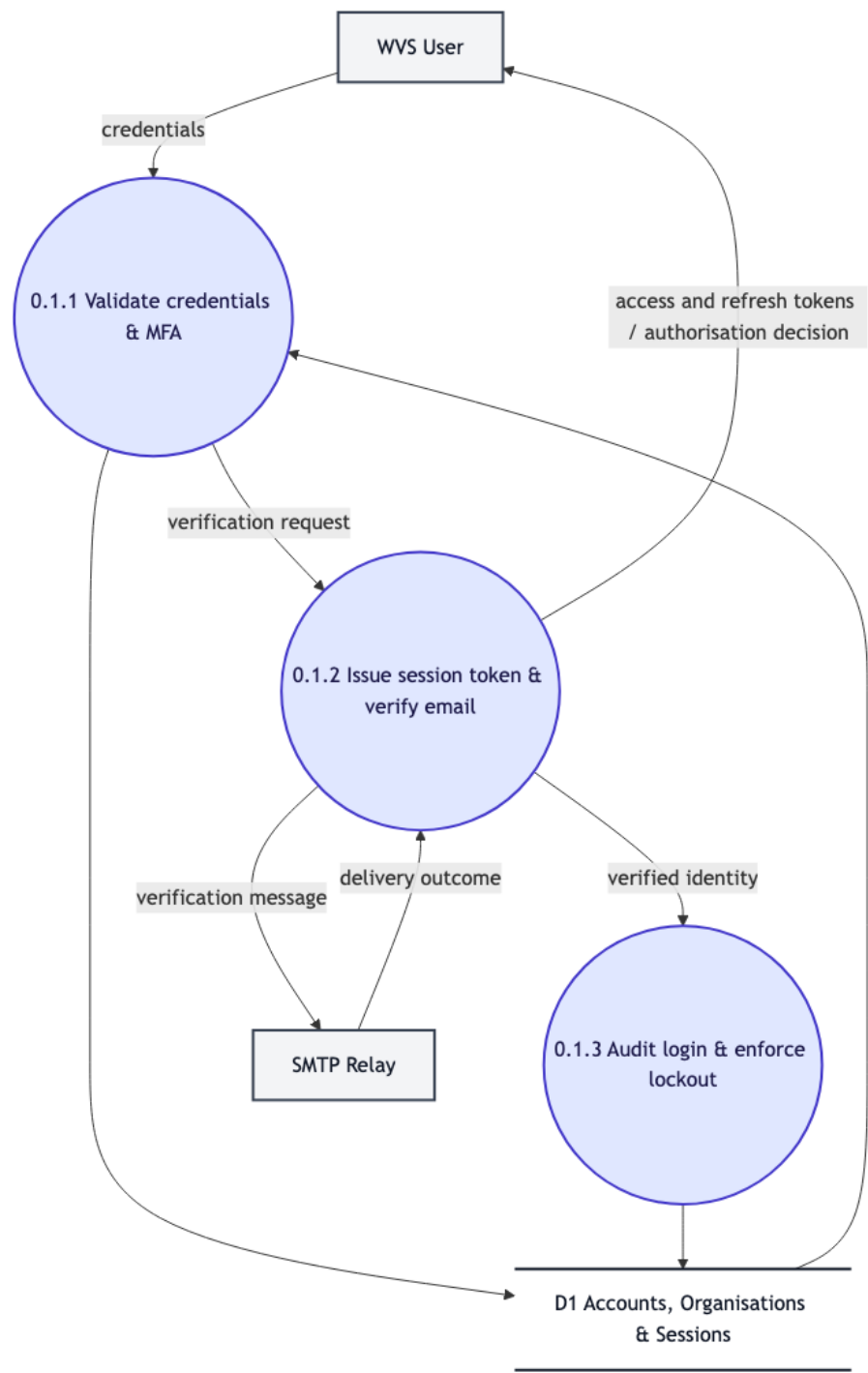
Figure 3: Level 2 DFD for 0.1 User Authentication & Access Control
