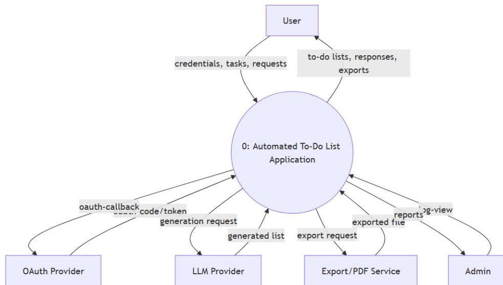
Figure 1: Level 0 Context Diagram
