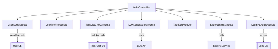
Figure 10: Level 1 Structure Chart of the System
