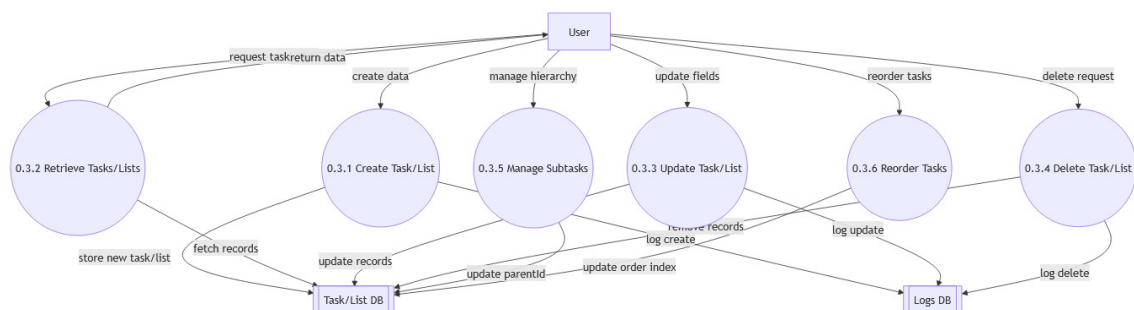
Figure 5: Level 2 DFD for 0.3 Task & List Management (CRUD)
