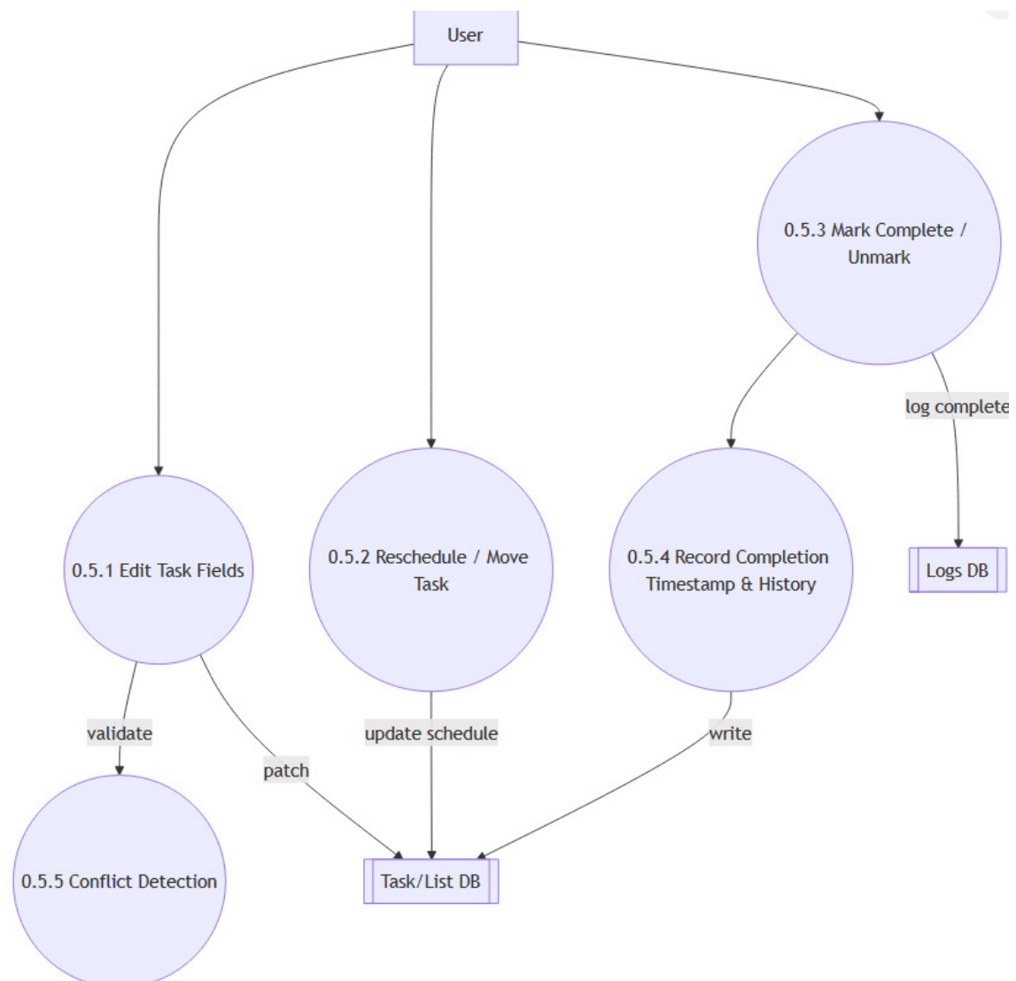
Figure 7: Level 2 DFD for 0.5 Task Editing & Completion
