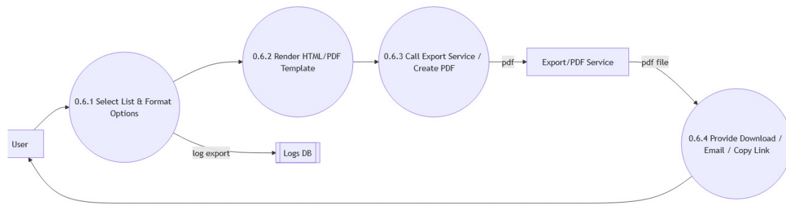
Figure 8: Level 2 DFD for 0.6 Exporting & Sharing
