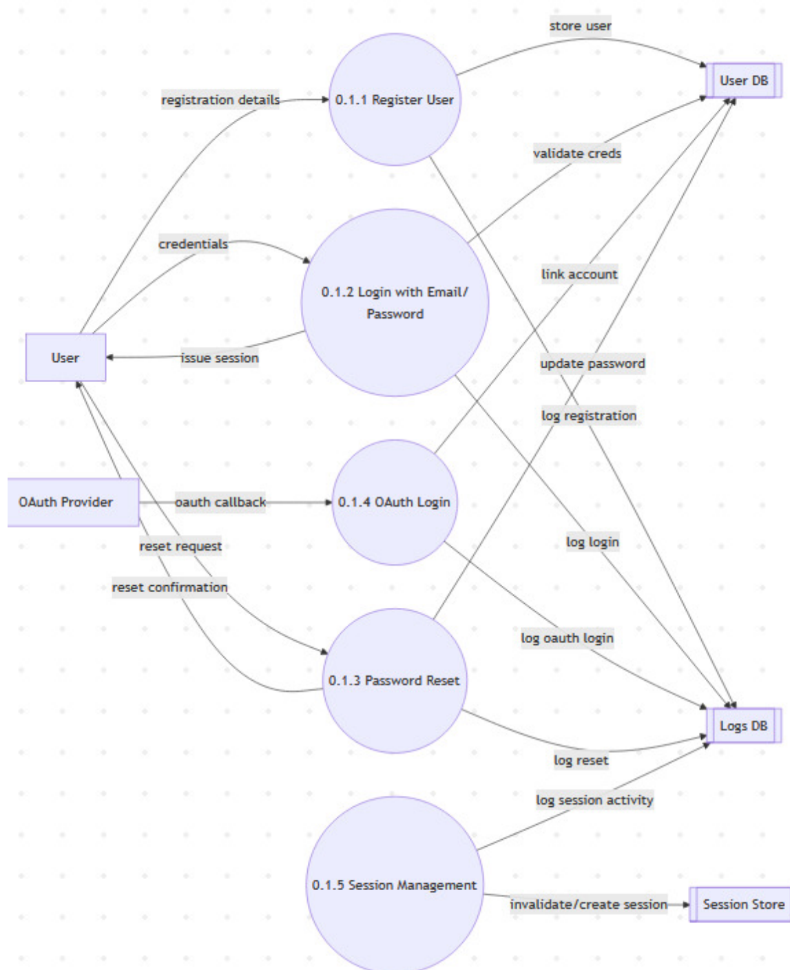
Figure 3: Level 2 DFD for 0.1 User Authentication & Management
