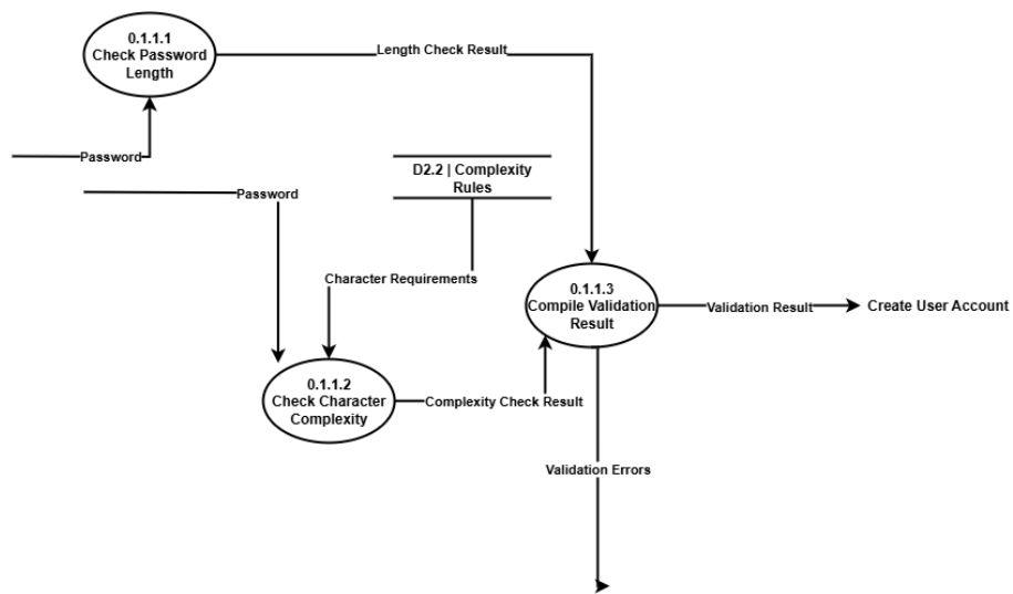
Level 3 DFD - Password Strength Validation
