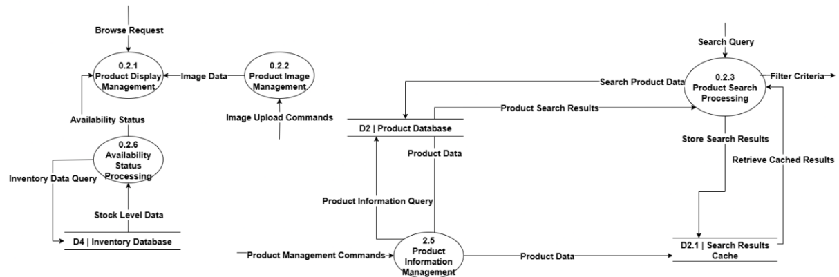
Level 2 DFD for Product Catalog Management
