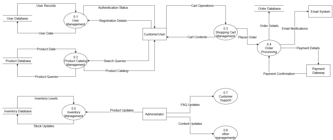
Level 1 Data Flow Diagram
