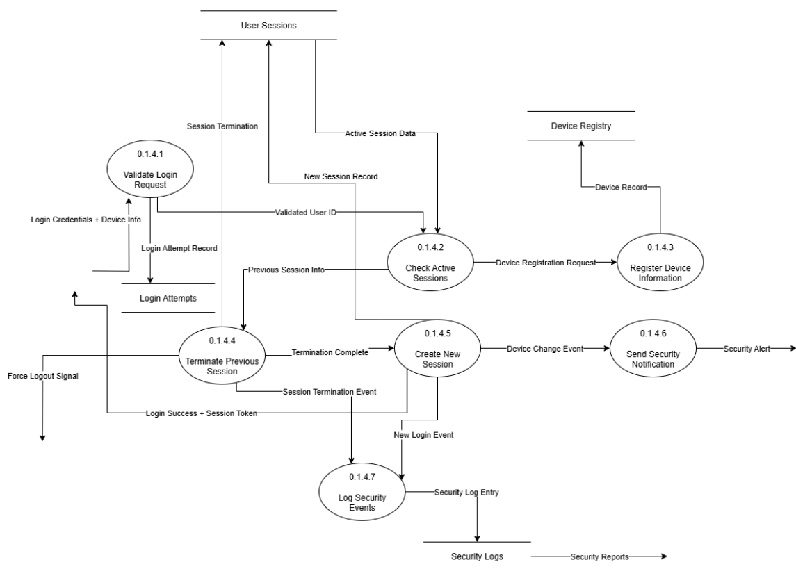
Level 3 DFD - Device Session Management
