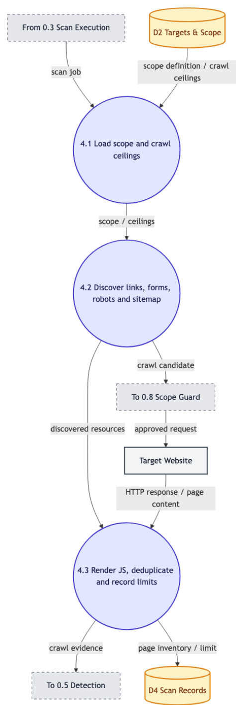
Figure 6: Level 2 DFD for 0.4 Discovery (Crawling)
