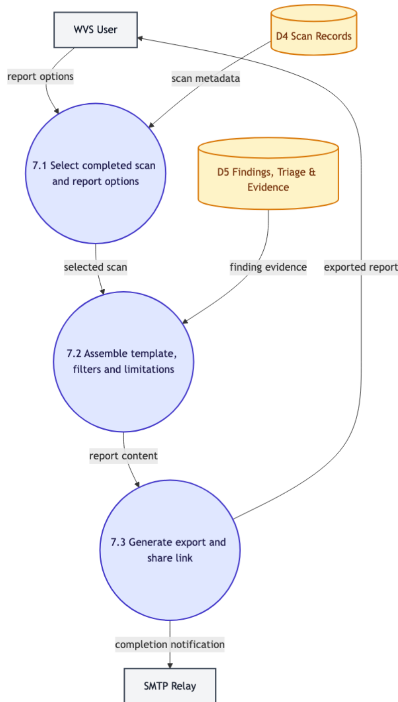
Figure 9: Level 2 DFD for 0.7 Reporting & Export
