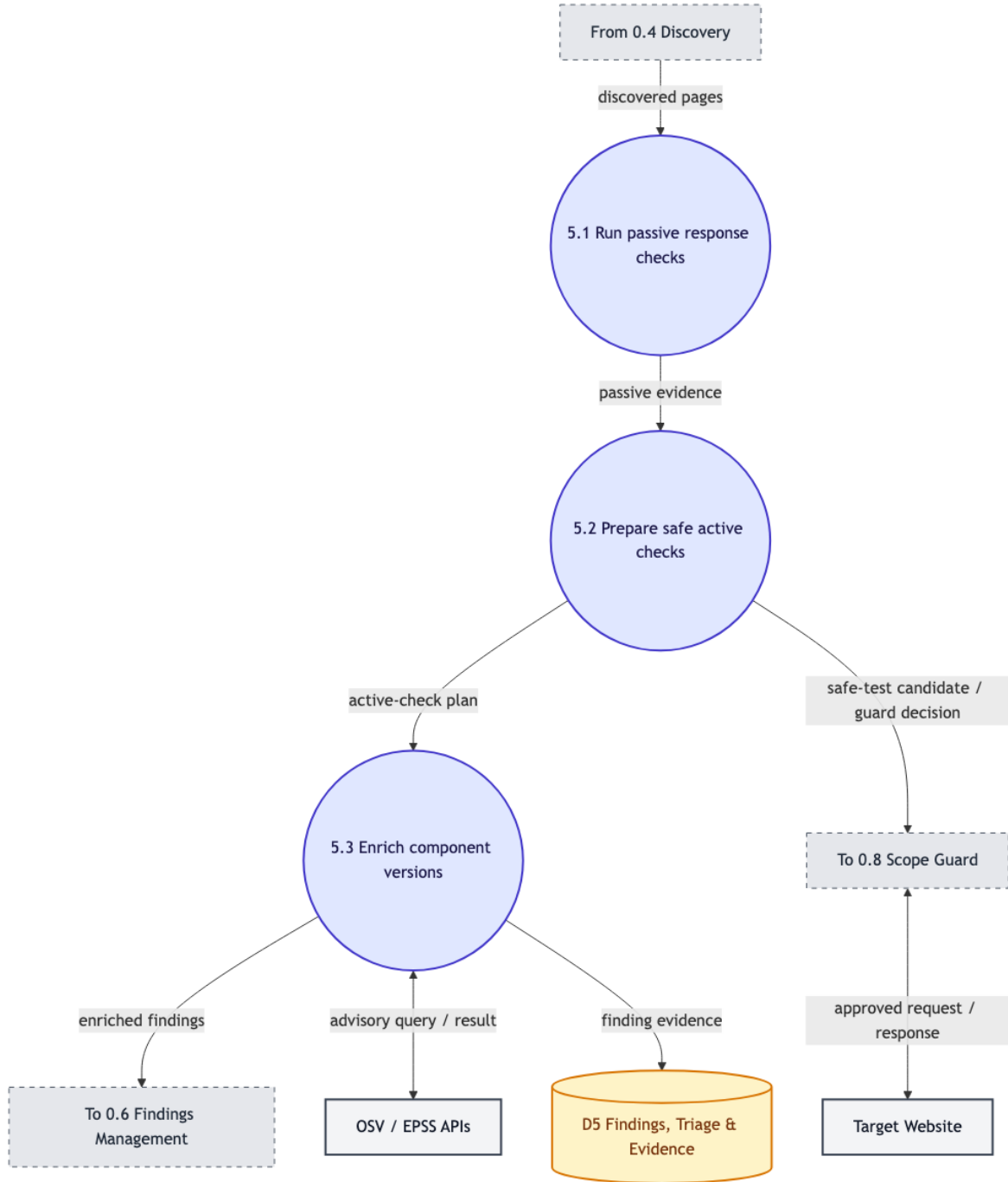
Figure 7: Level 2 DFD for 0.5 Vulnerability Detection
