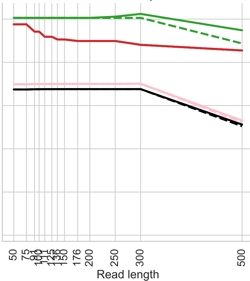
dataset = rye
