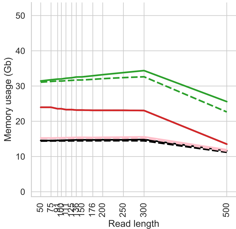
dataset = CHM13
