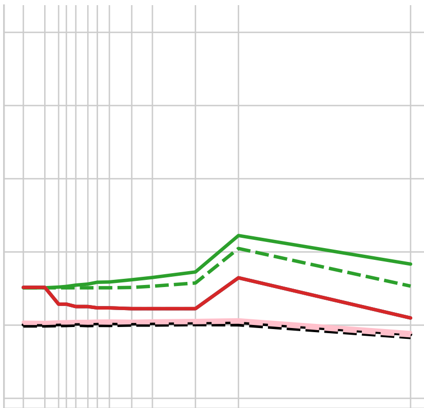
dataset = maize
