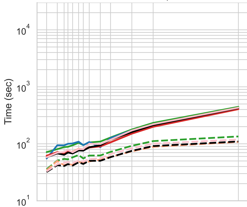
dataset = drosophila
