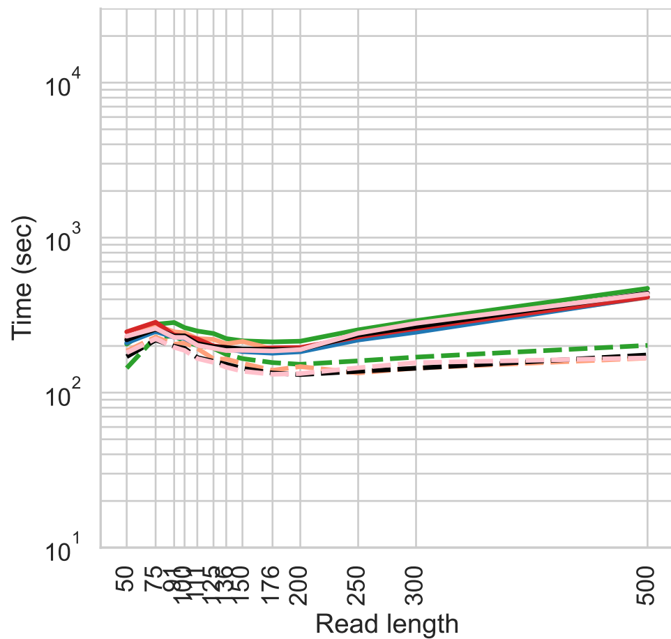
dataset = CHM13
