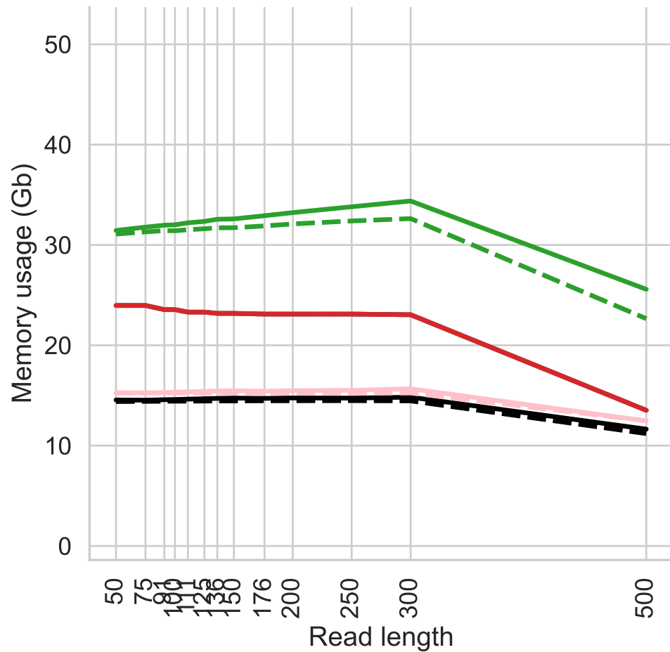
dataset = CHM13
