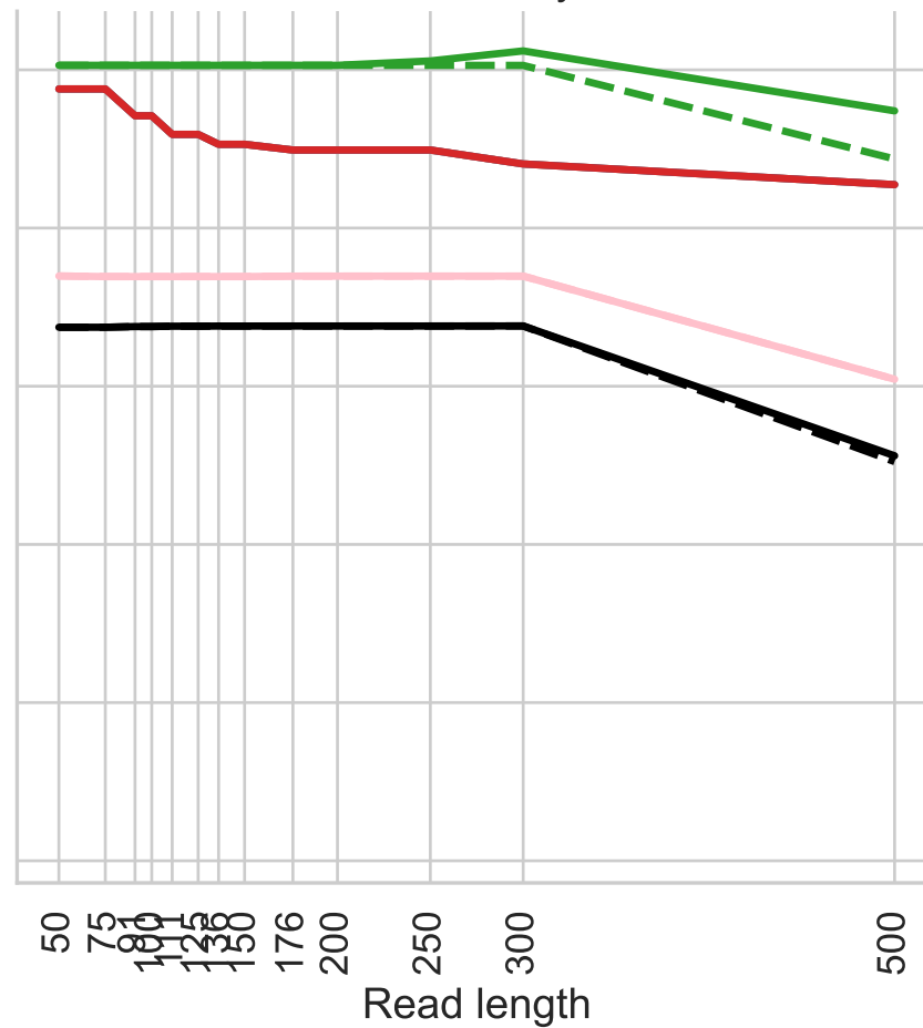
dataset = rye
