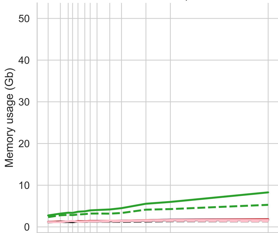
dataset = drosophila
