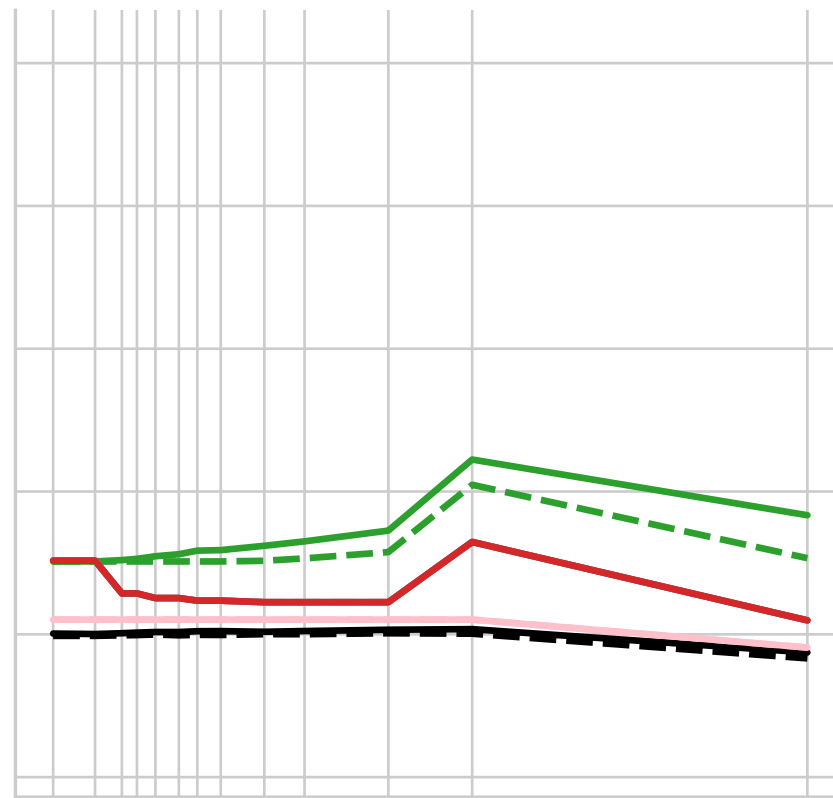
dataset = maize
