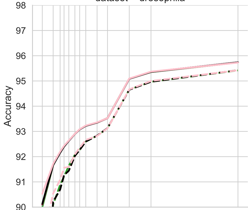
dataset = drosophila
