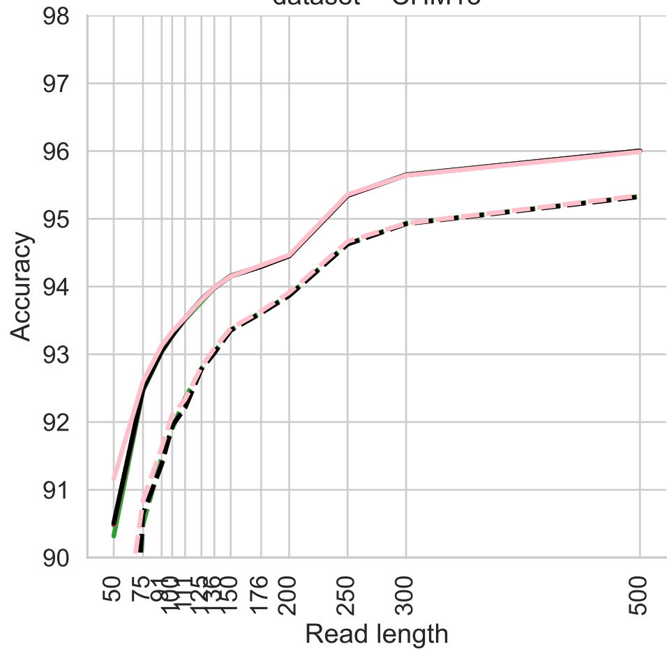
dataset = CHM13
