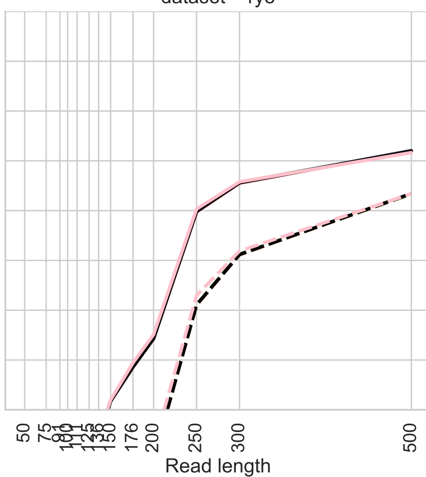
dataset = rye
