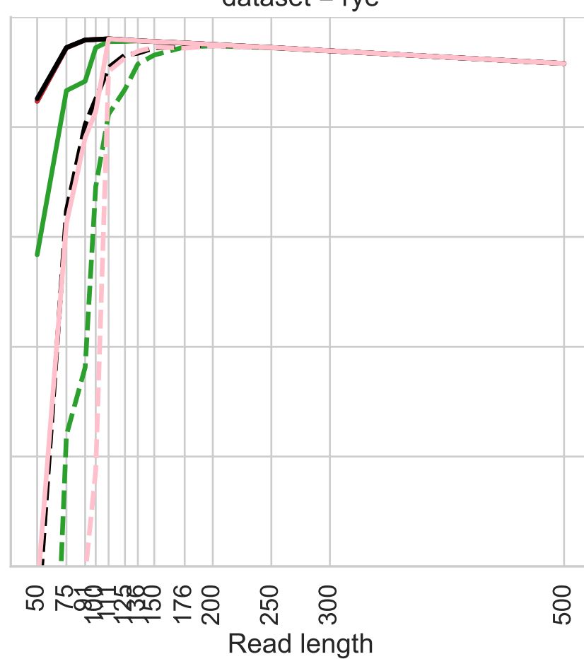
dataset = rye
