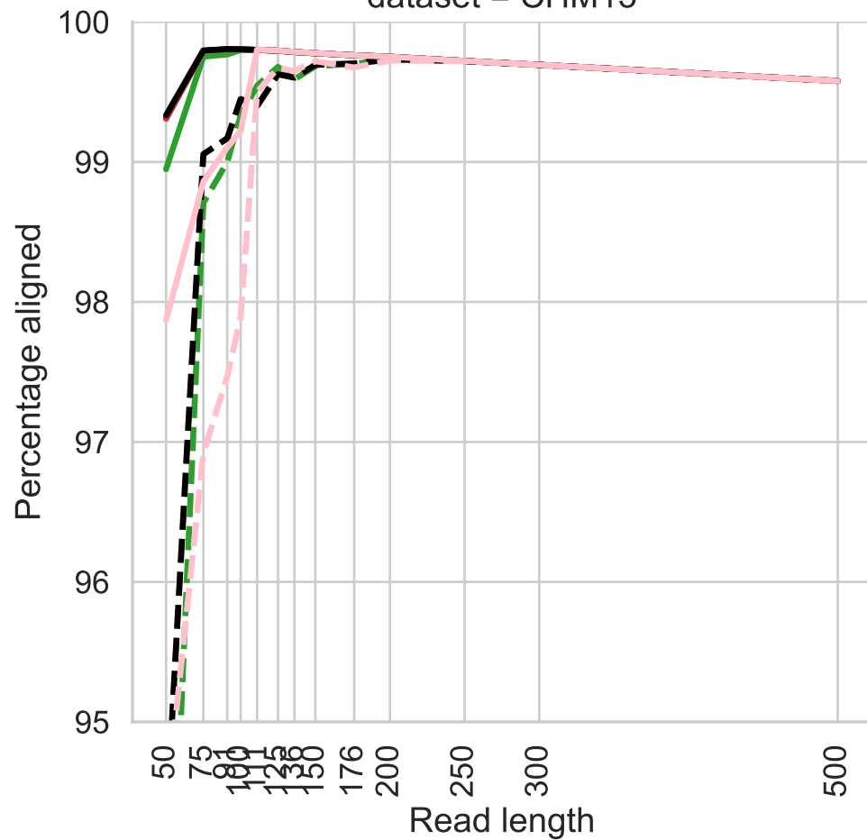
dataset = CHM13
