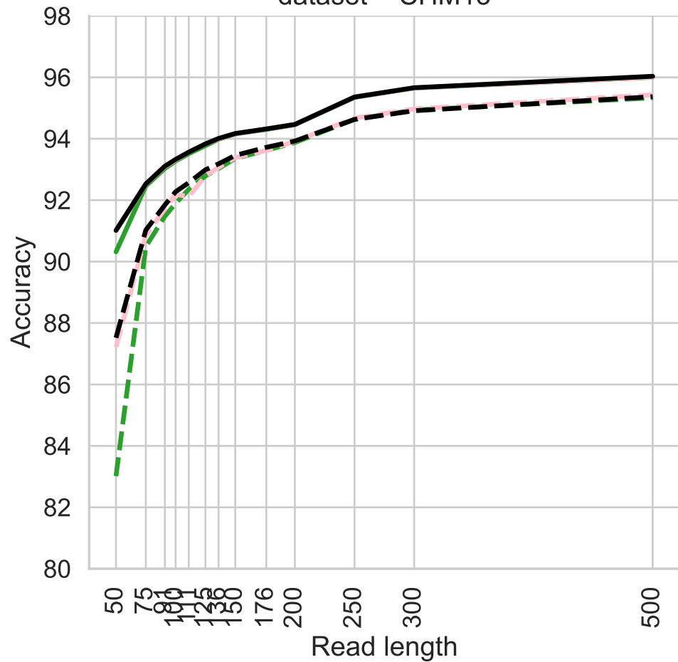
dataset = CHM13
