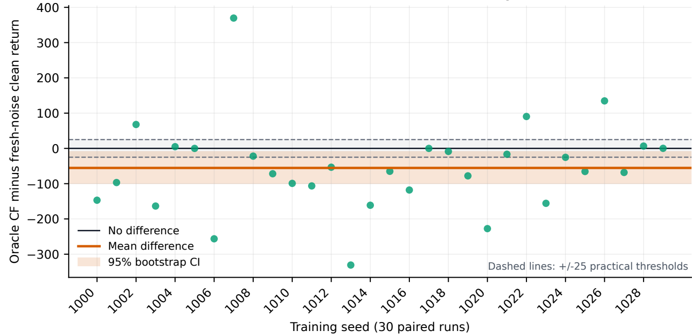
Paired clean-return differences across training seeds
