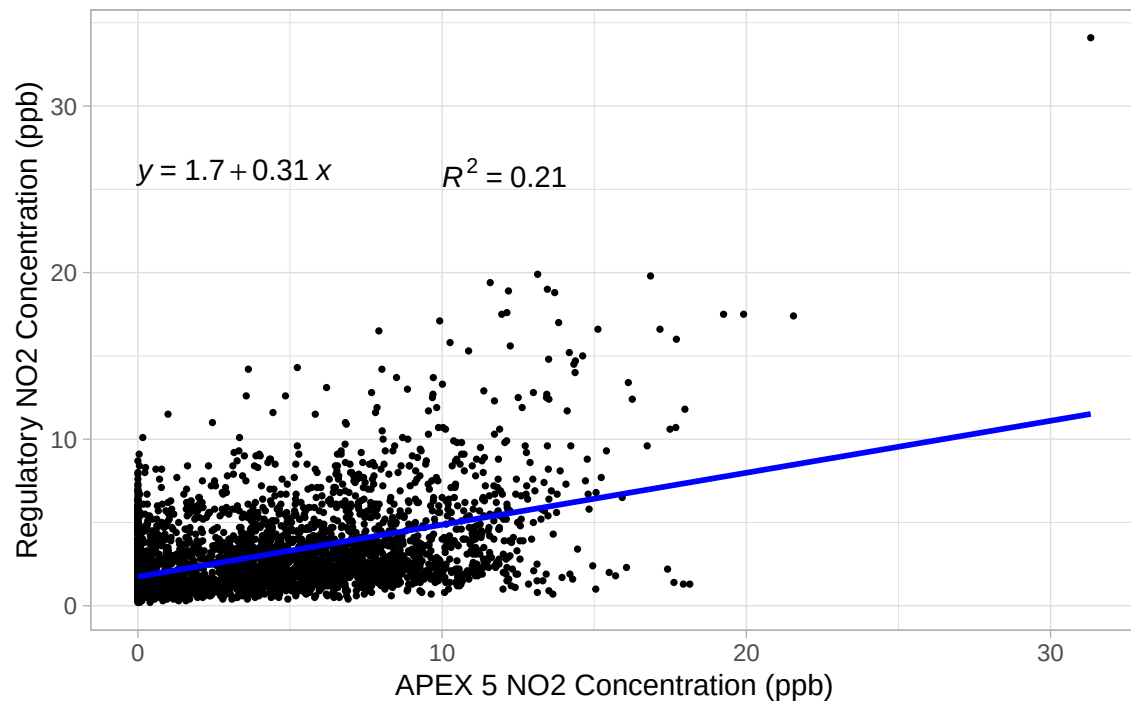
Broad Run HS: NO2 APEX 5 Sensor vs Regulatory Monitor
