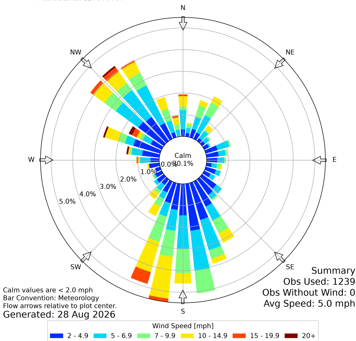
Figure 3: Wind Rose from Dulles Airport.
