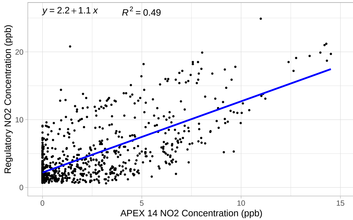
Broad Run HS: NO2 APEX 14 Sensor vs Regulatory Monitor
