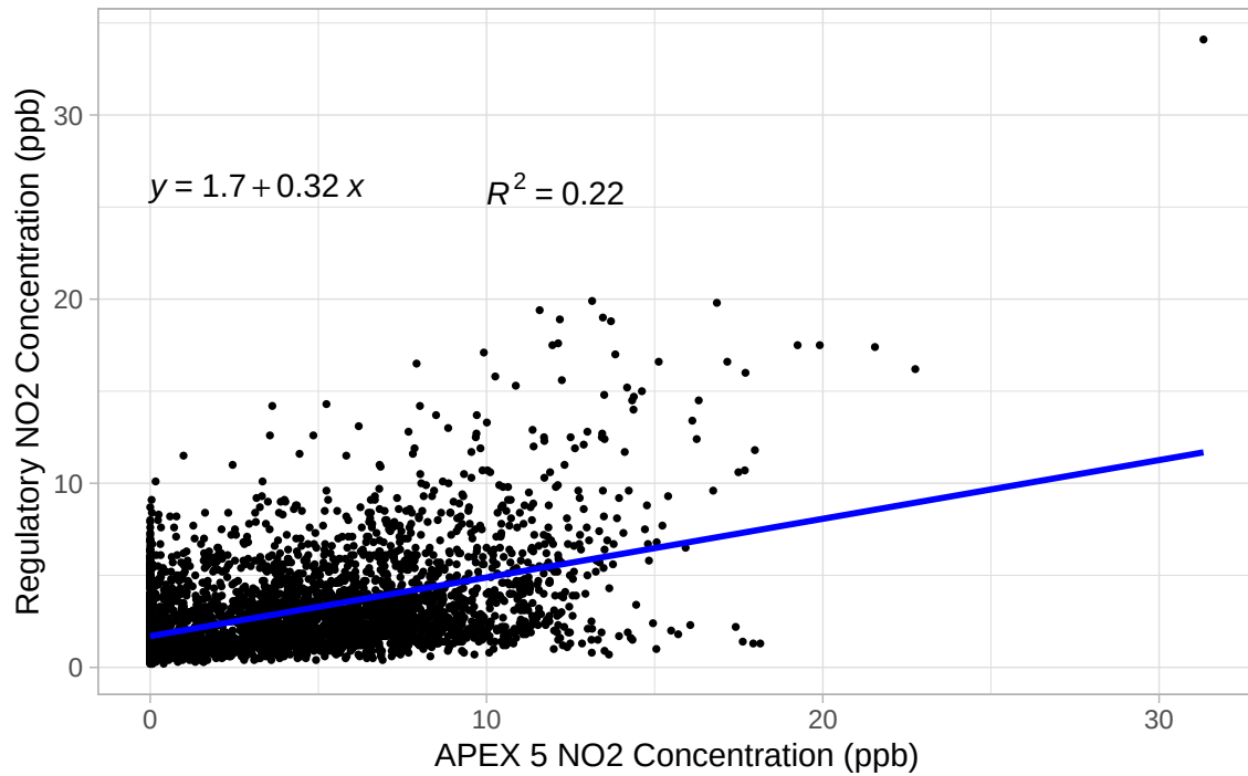
Broad Run HS: NO2 APEX 5 Sensor vs Regulatory Monitor
