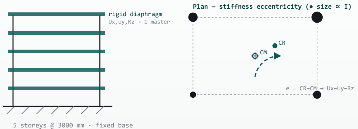
Figure SM5b. Eccentric multi-storey building — rigid floor diaphragms (elevation) and the plan stiffness eccentricity (• size ∝ I) that offsets CR from CM and couples the Ux-Uy-Rz response.
