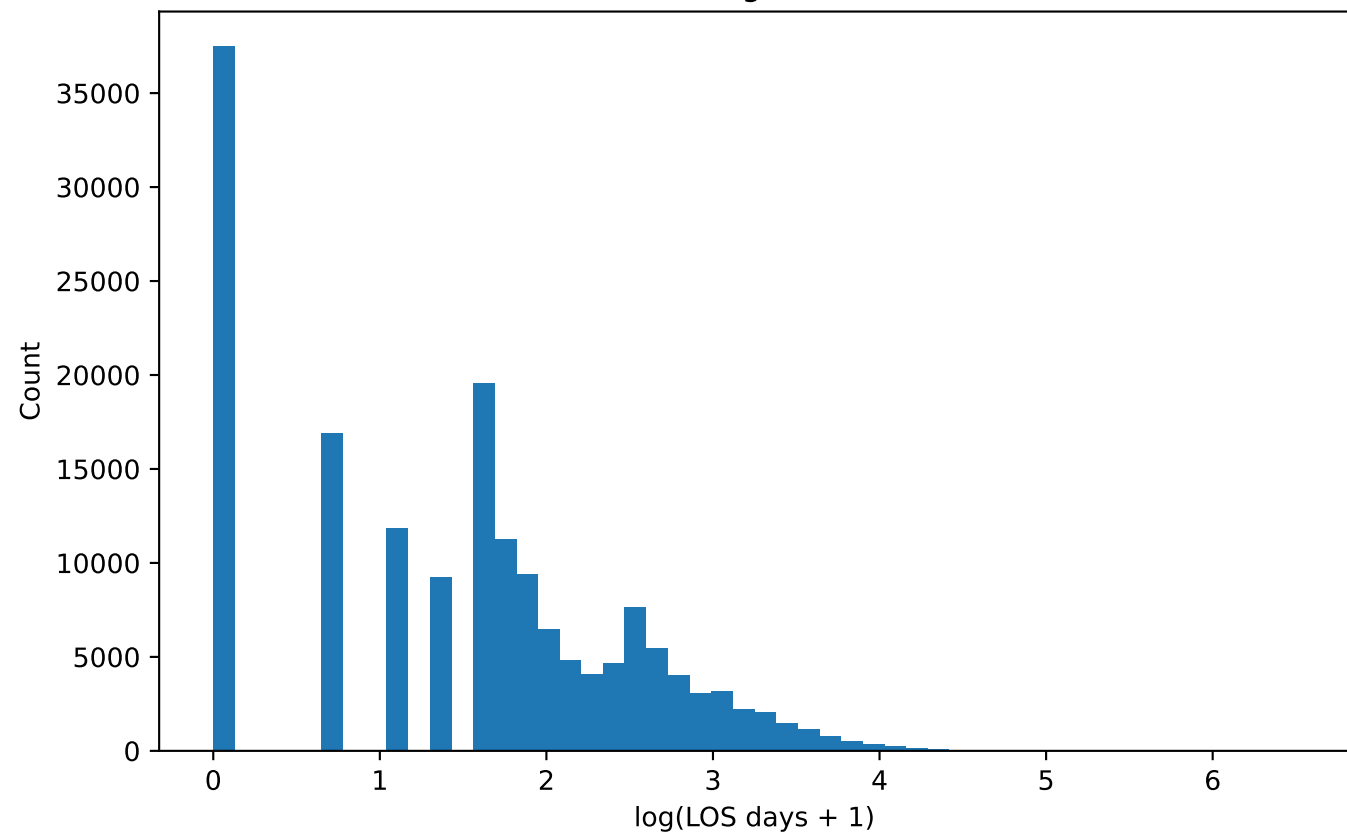
Distribution of Log-transformed LOS
