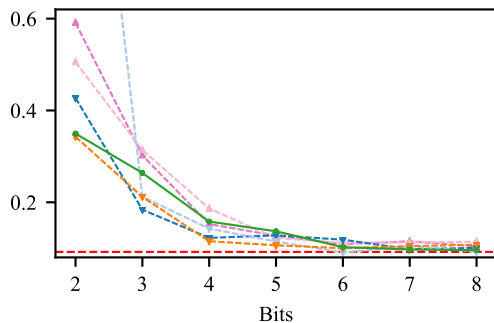
sulfur
