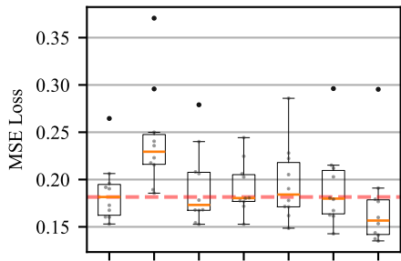
cpu_act
