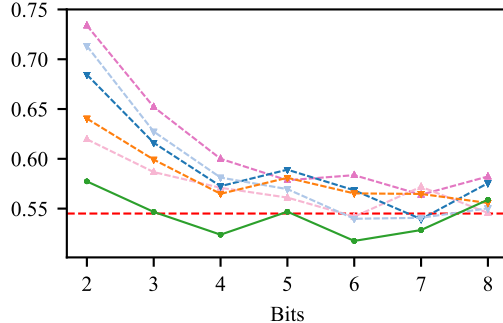
wine_quality
