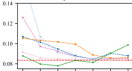
wine_quality
