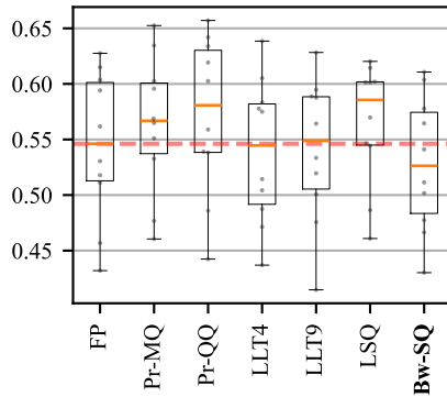
wine_quality
