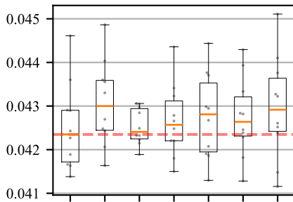
sulfur
