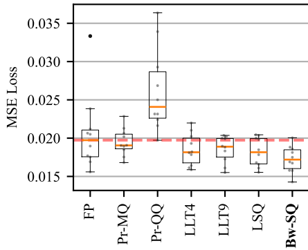
cpu_act
