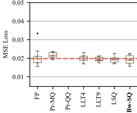
cpu_act
