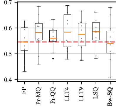
wine_quality
