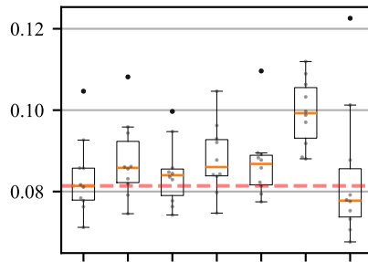
wine_quality
