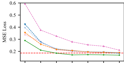
cpu_act
