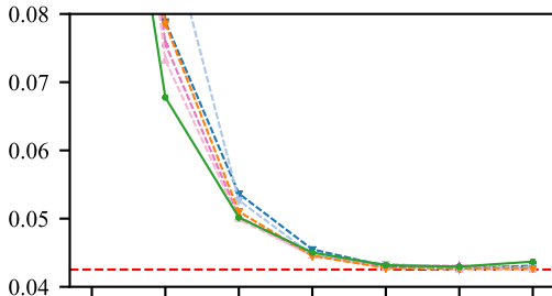
sulfur
