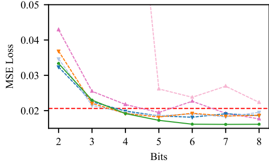
cpu_act
