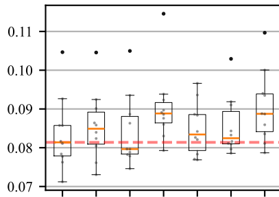
wine_quality
