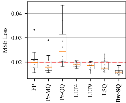
cpu_act
