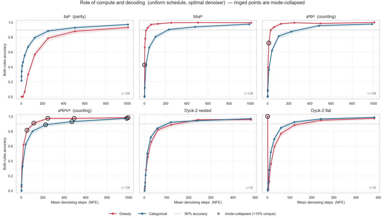
Figure 1: Both-rules accuracy vs. realised mean denoising steps (NFE) under the uniform schedule with the optimal denoiser. Greedy (red) vs. categorical (blue); ribbons are the pooled 95% Wilson confidence interval; the dotted line marks 90% accuracy. Ringed points are mode-collapsed (uniqueness < 10%): a high-accuracy ring is a single repeated valid string, not skill. Each panel annotates its sequence length L .
