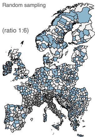
Random sampling
