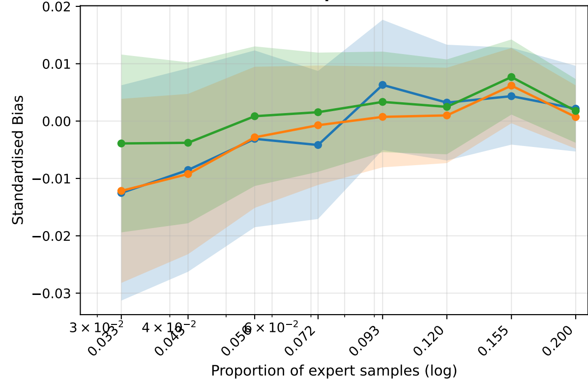
Mistral
