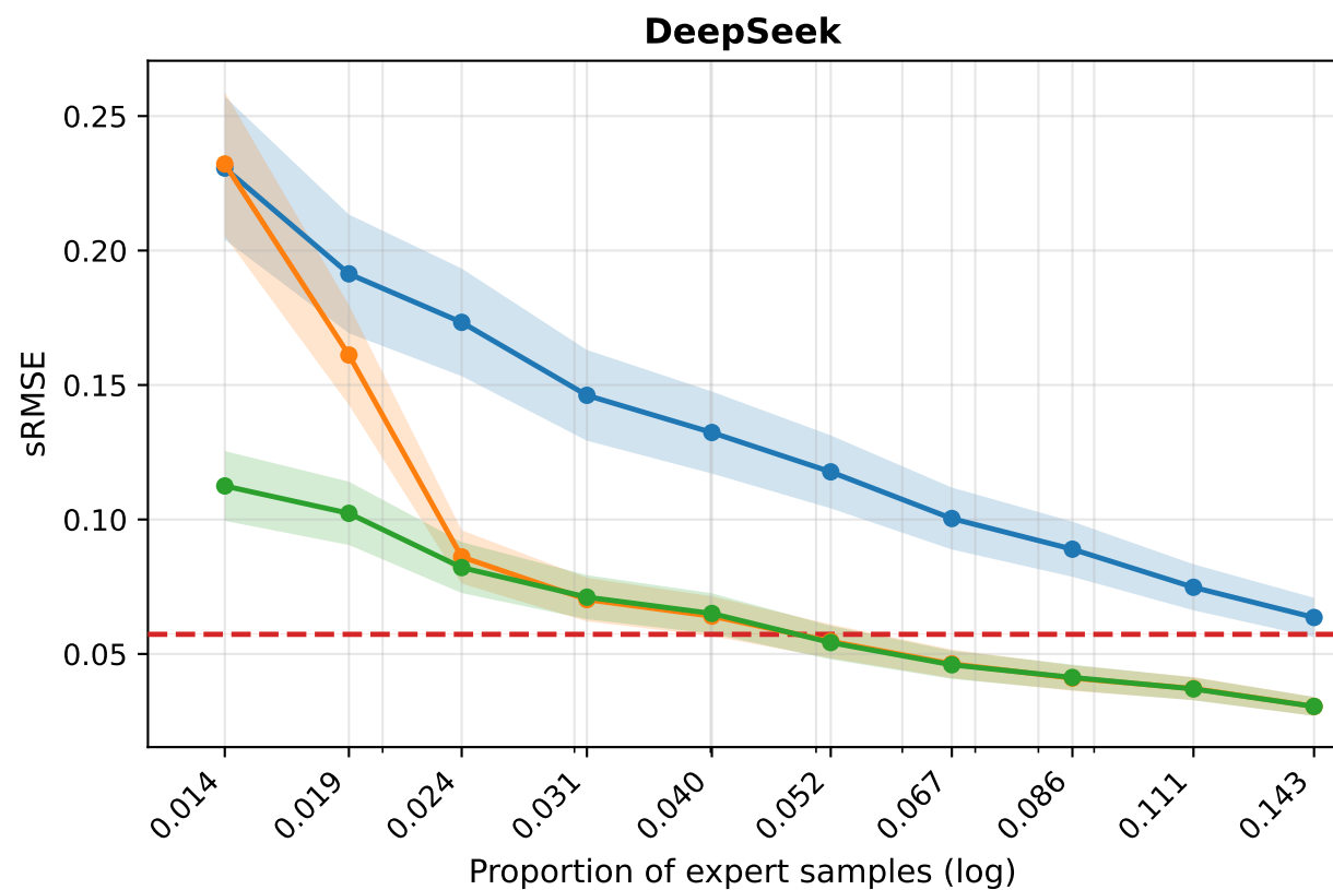
Class Prevalence — sRMSE with LLM baseline (CUAD)
