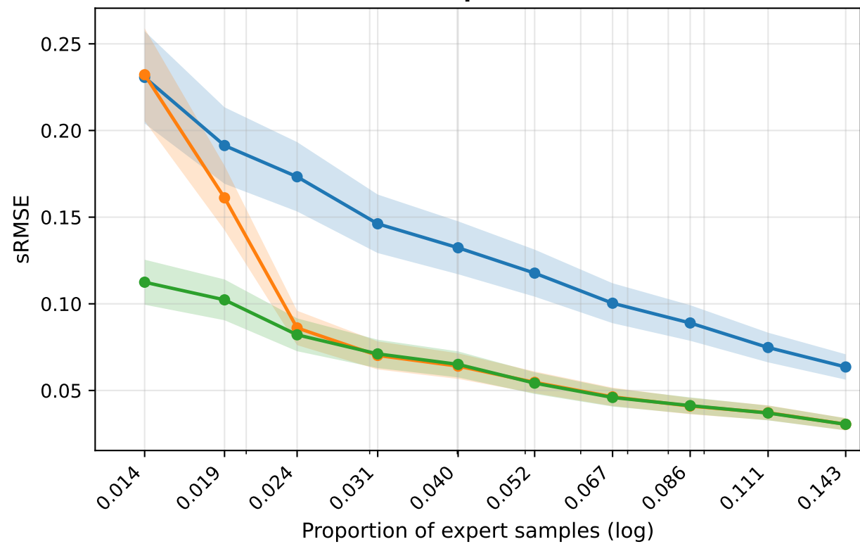
Mistral
