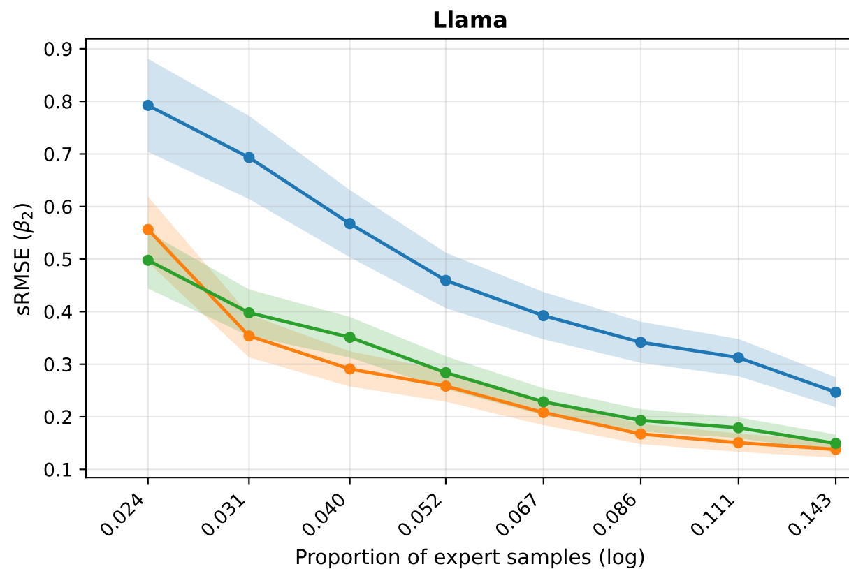
Low-Variance Feature — sRMSE of \beta_2 (CUAD)
