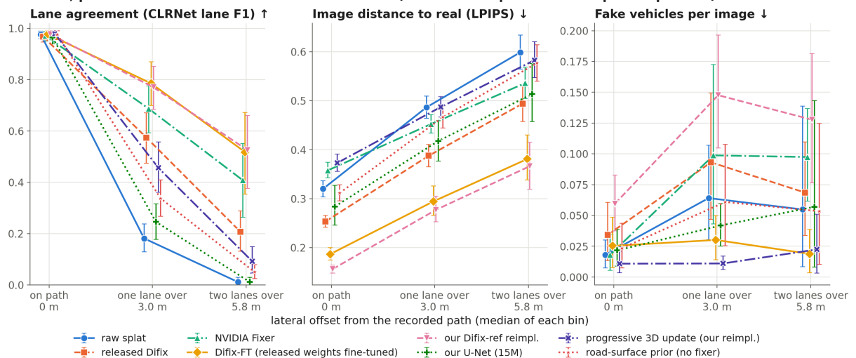
Figure 1. Lane agreement, perceptual distance and spurious vehicles against lateral offset, pooled over eight held-out roads.
