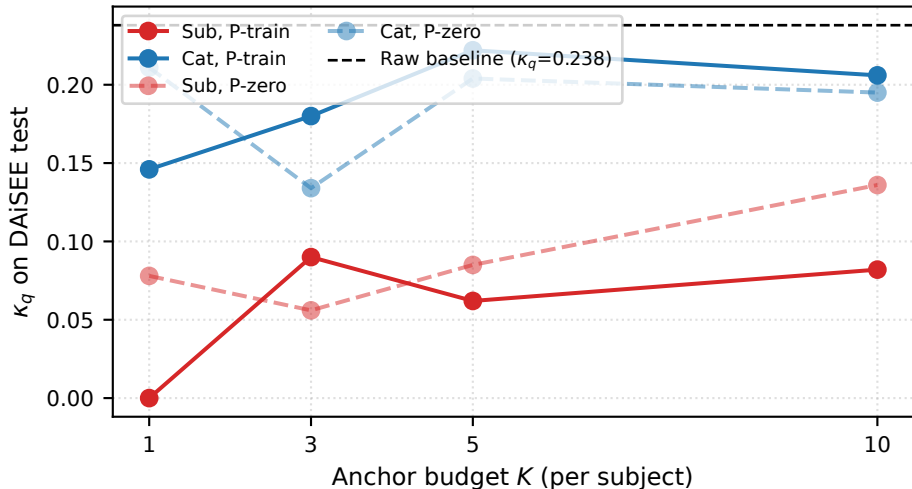
DREAM: \kappa_q vs anchor budget
