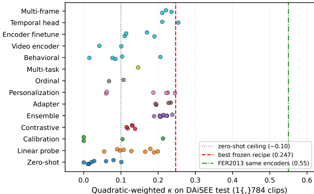
Method-family landscape: 50+ frozen-feature variants on DAiSEE
