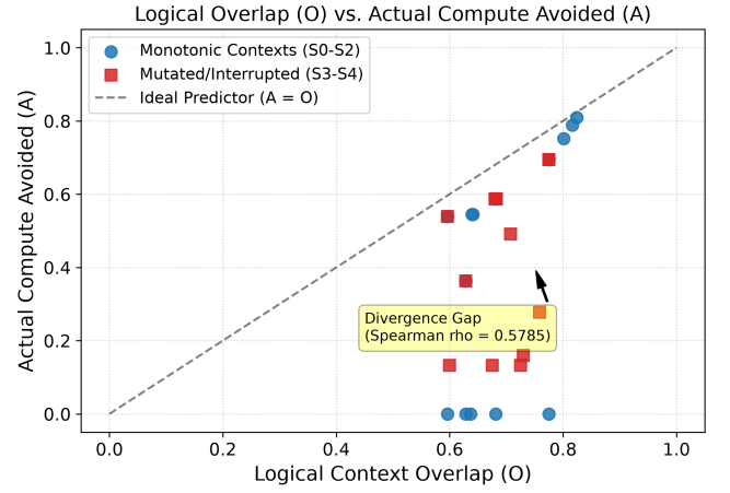
Fig. 1. Logical Context Overlap ( O ) vs. Actual Compute Avoided ( A ). Under context mutations and pause decay, logical metrics severely overestimate actual compute avoided.
