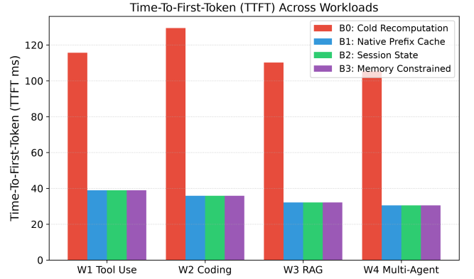
Fig. 2. Time-To-First-Token (TTFT) comparison between Cold Recomputation ( B_0 ) and Native Prefix Caching ( B_1 ) across workloads.
