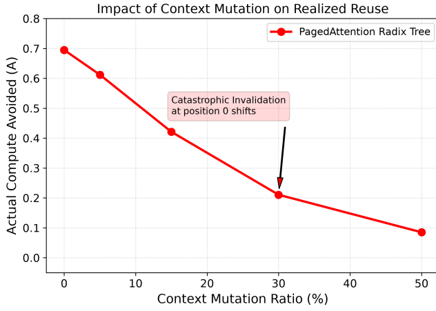
Fig. 3. Impact of context mutation ratio on Actual Compute Avoided ( A ). Small front/mid insertions cause catastrophic physical KV cache invalidation.
