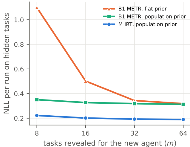
Prediction of hidden tasks
