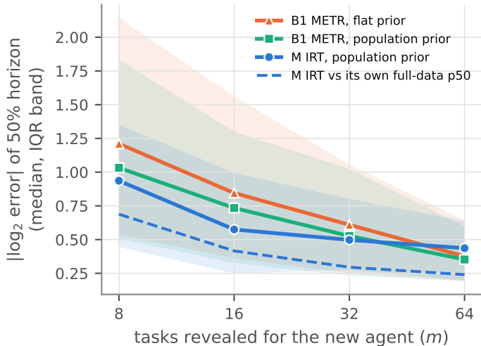
Horizon recovery (target: METR full-data p50)
