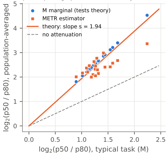
p50→p80 gap is stretched by s
