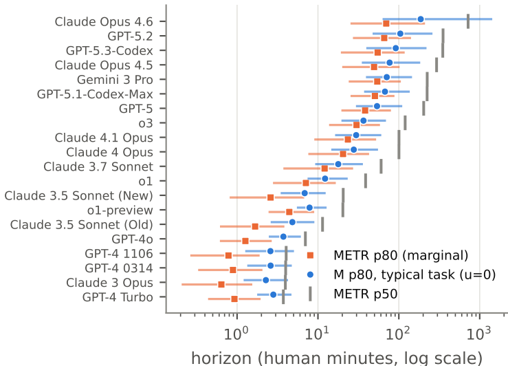
80% horizons: marginal vs typical task
