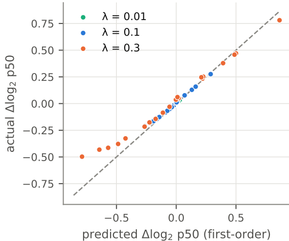
Ridge rotates curves about a pivot
