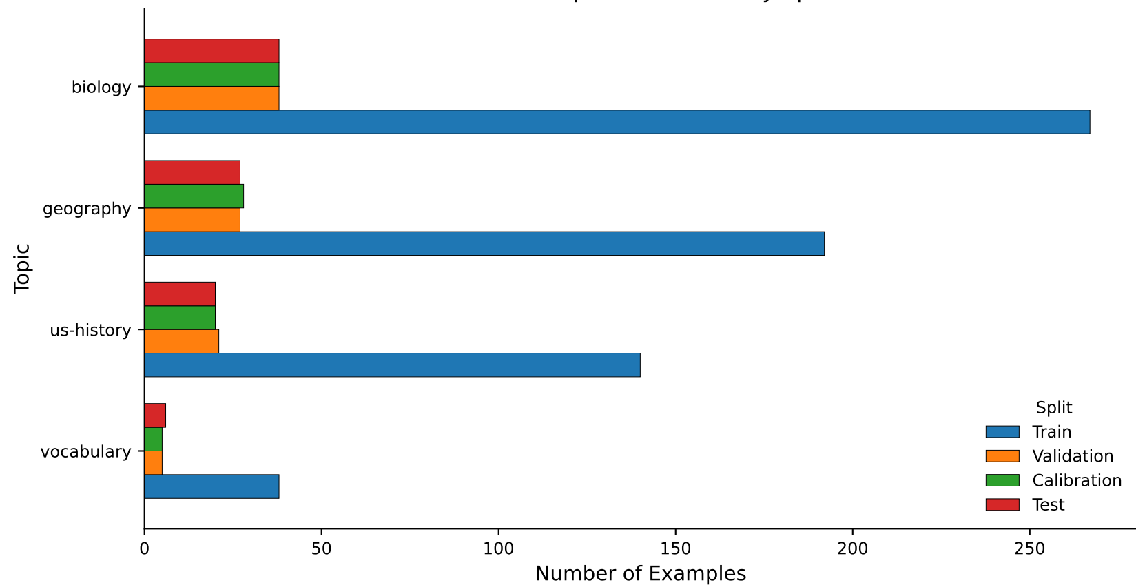
Client 1: Topic Distribution by Split
