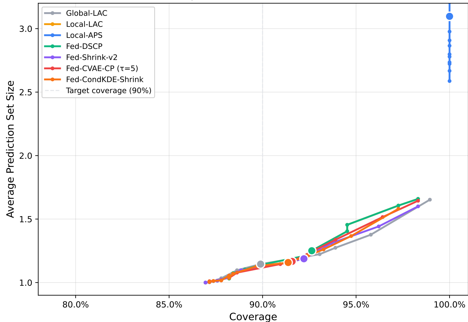
Coverage-Efficiency Trade-off (Pareto Curve) Lower-right is better. Filled dots = \alpha = 0.10 .
