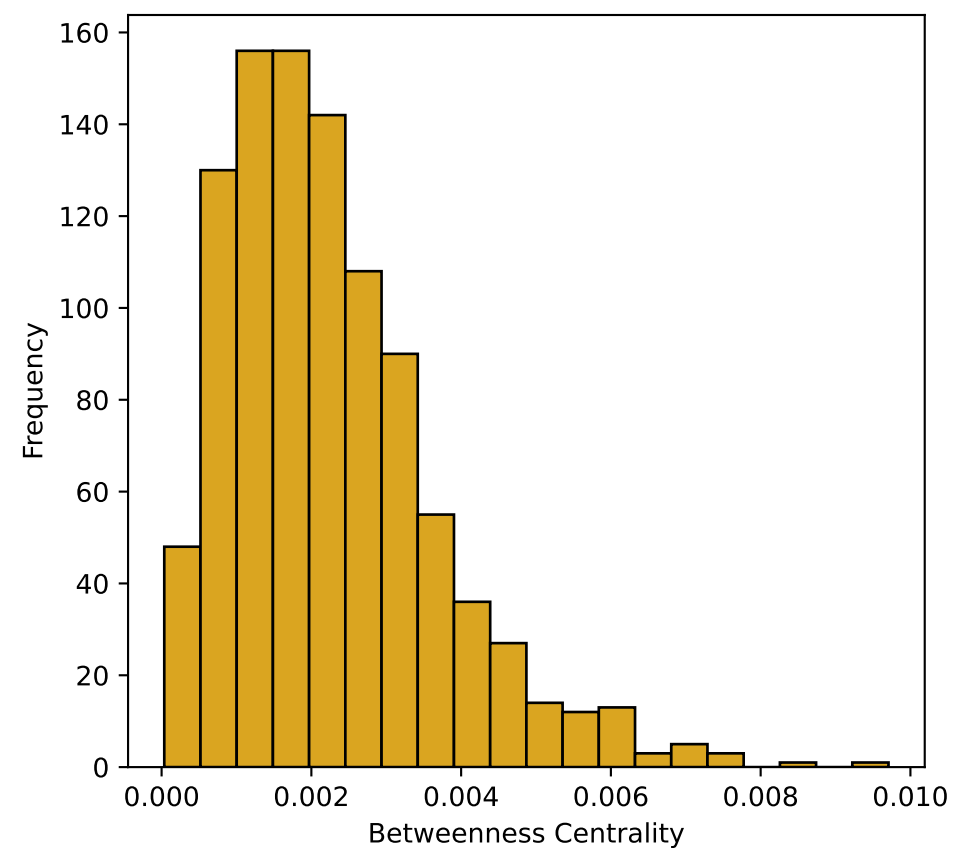
Degree and centrality distribution for Erdos-Renyi graph with N = 1000
