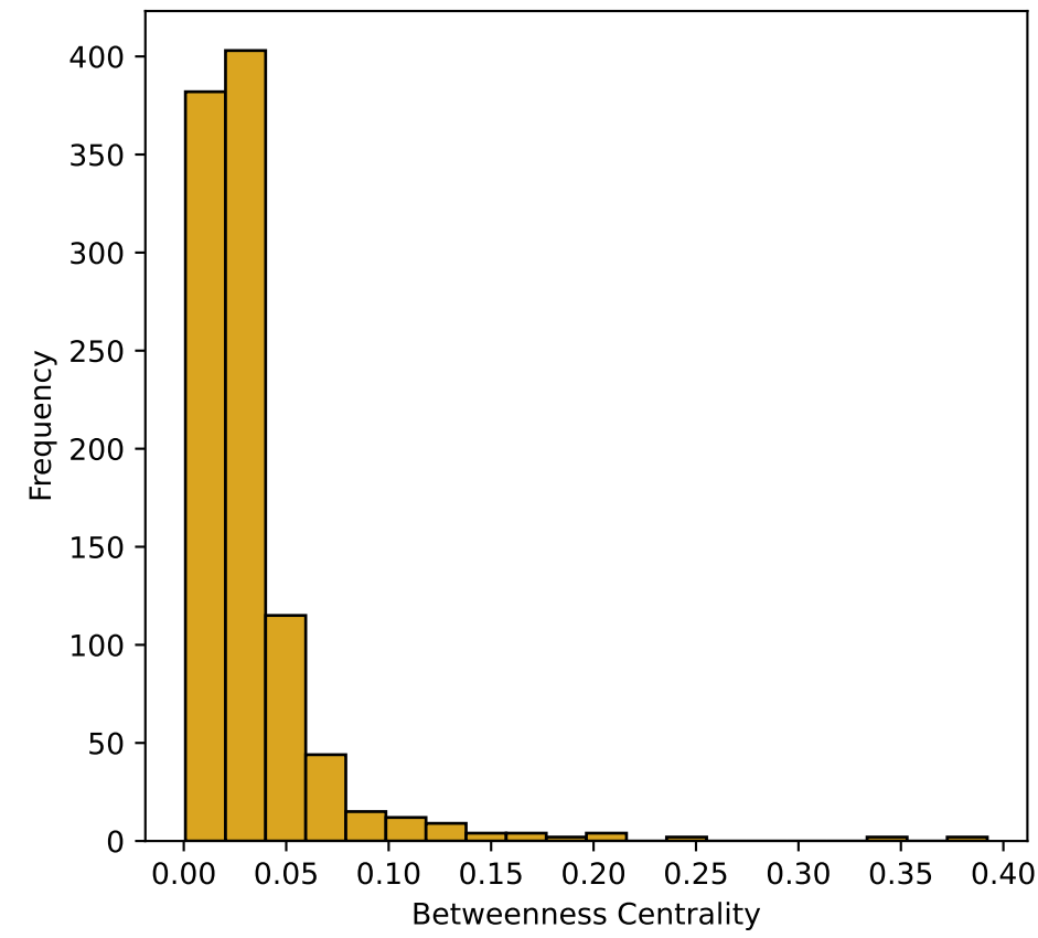
Degree and centrality distribution for Watts-Strogatz graph with N = 1000
