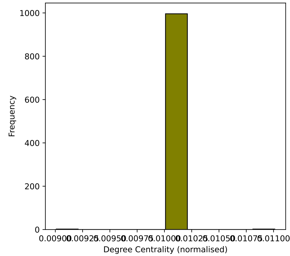
Degree and centrality distribution for Watts-Strogatz graph with N = 1000
