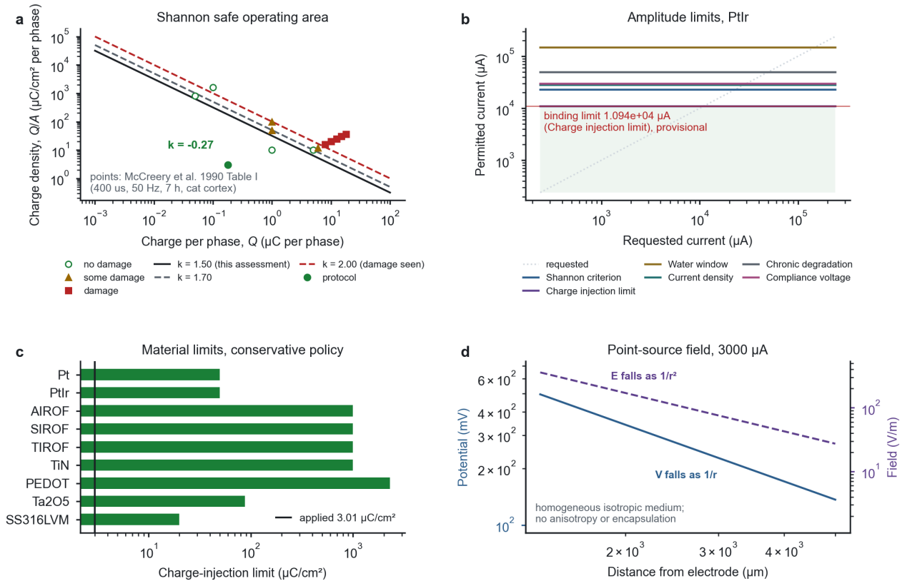
Fig. 2. Output of neurostim-safety for a DBS contact (3 mA, 60 \mu\text{s} per phase, 130 Hz, in vivo). (a) The protocol on the Shannon safe-operating plane with McCreery's data. (b) Permitted current per check against requested current, with the binding limit. (c) Material charge-injection limits under the conservative policy. (d) Potential and field around the contact.
