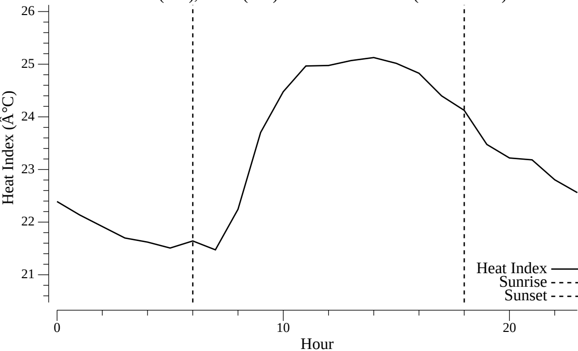
24h Heat Index (7-day hourly averages) - Paphos Walk: 06:00 (~2h), 18:00 (~1h) Avoid: 12:00-11:59 (Asia/Nicosia)
