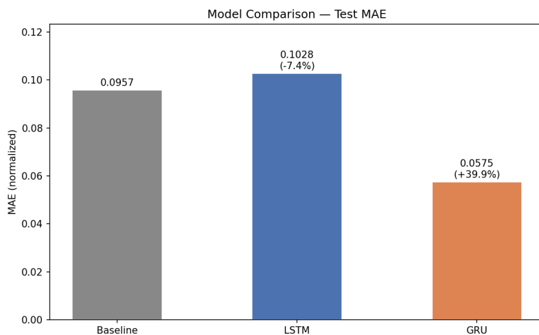
Figure 2: Test MAE for the baseline, best LSTM, and GRU on Run 1 (2023 data, 14k sequences). The GRU achieves a 39.9% improvement over the moving average baseline; the default LSTM slightly underperforms it.
