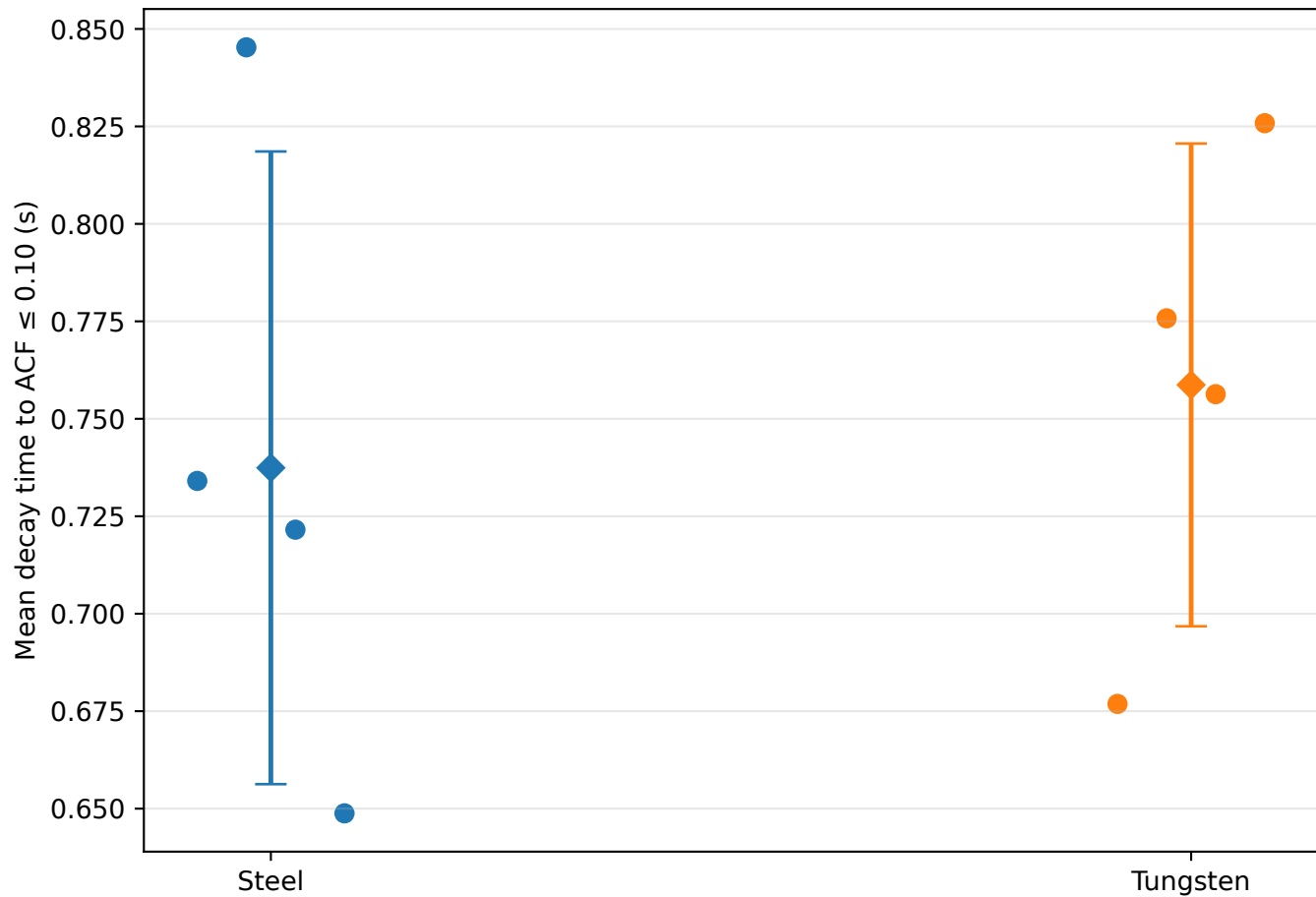
Autocorrelation decay time
