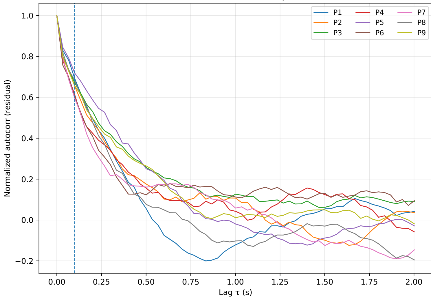
Autocorrelation curves for 9 fixed patches: steel
