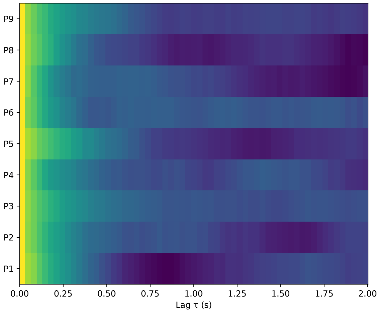
Autocorrelation map: 9 fixed patches \times lag (steel)
