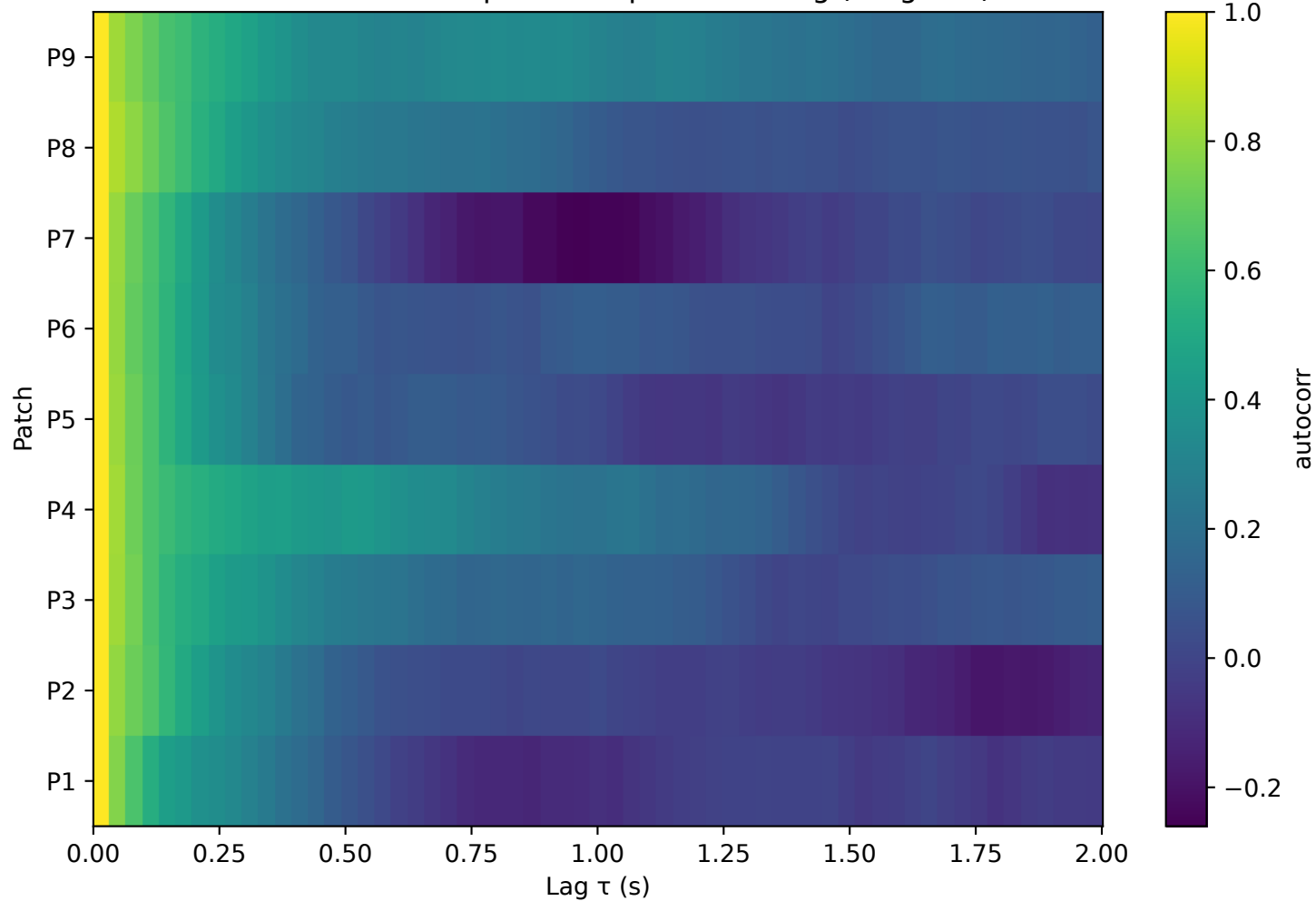
Autocorrelation map: 9 fixed patches \times lag (tungsten)
