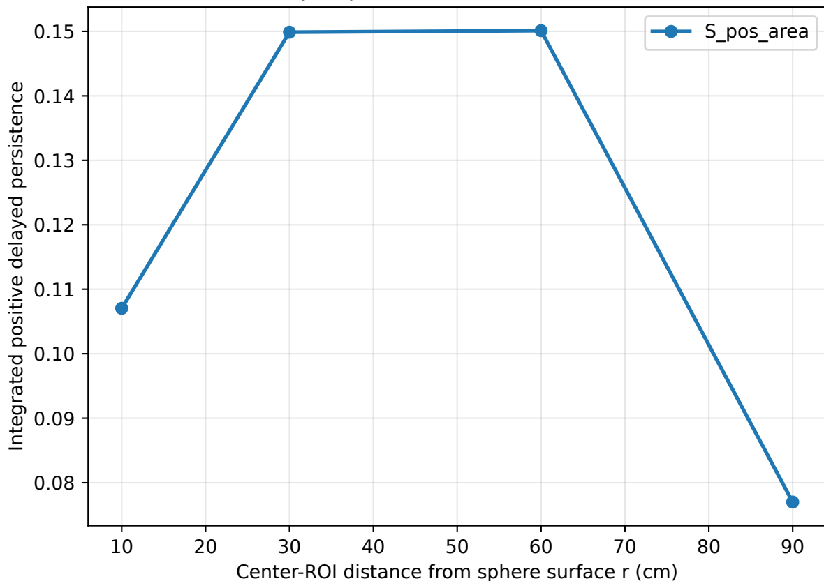
Positive delayed persistence area vs distance: hollow
