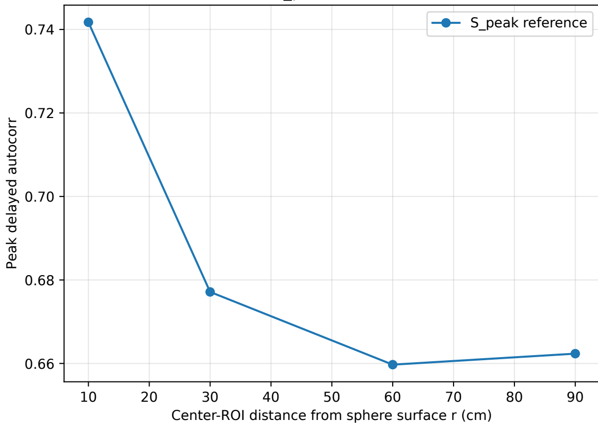
Reference S_peak vs distance: solid
