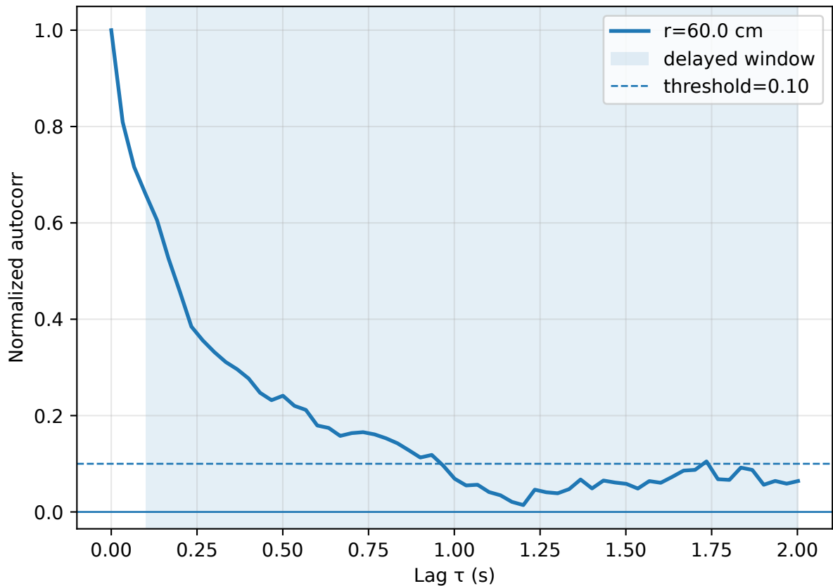
Center-ROI temporal persistence, r=60.0 cm
