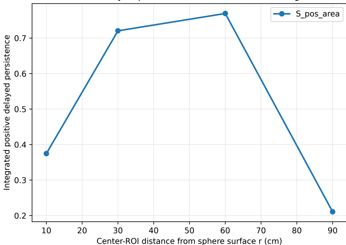
Positive delayed persistence area vs distance: tungsten
