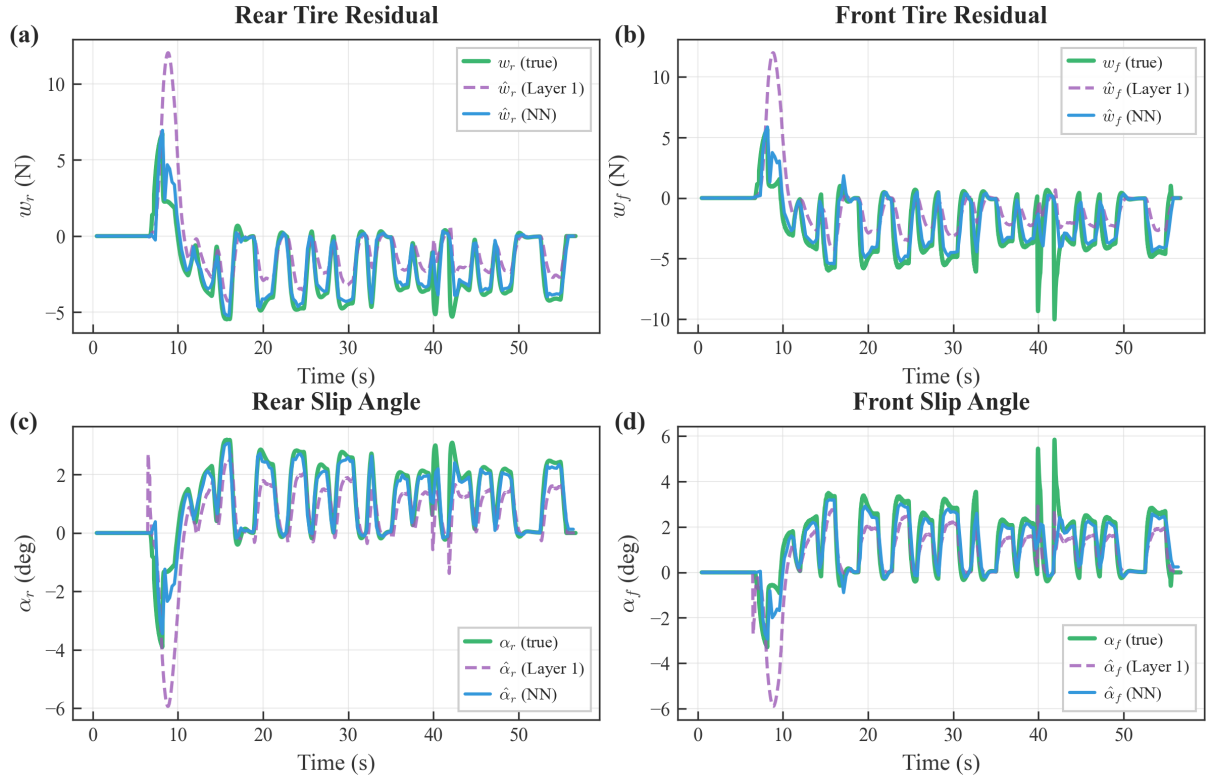
Figure 3.5: Tire-force residual and slip angle estimation: Layer 2 (NAO) achieves faster convergence and higher precision compared to Layer 1 (UO), while both estimates remain bounded.
