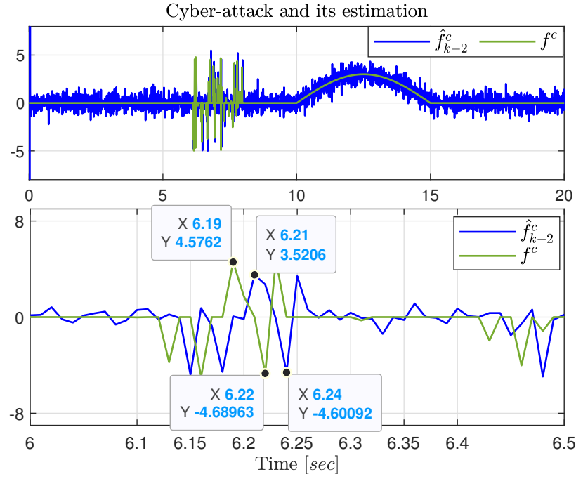
Figure 2.5: Attack estimation using UIO case 1.
