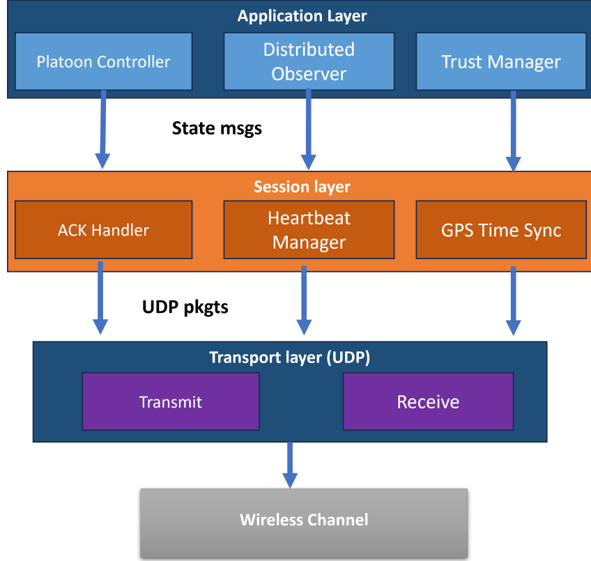
Figure 5.4: Layered architecture of the V2V communication stack used in the QLab experiments.
