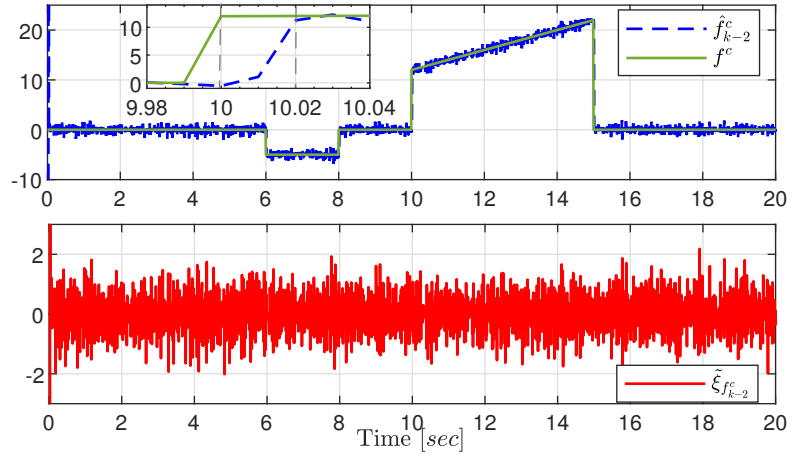
Figure 2.6: Attack estimation and the errors case 2.
