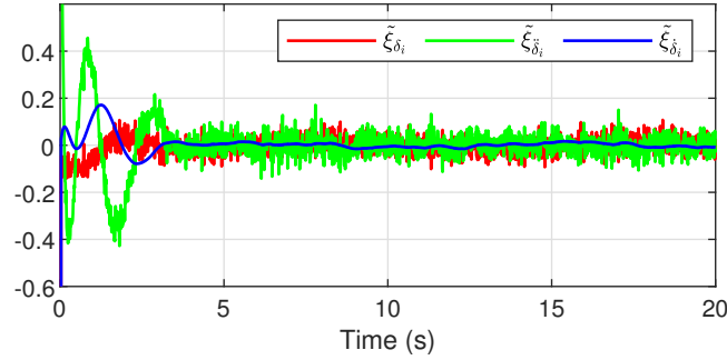
Figure 2.4: State estimation case 1.
