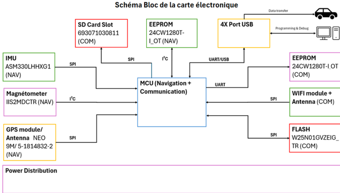
Figure 5.7: Block architecture.
