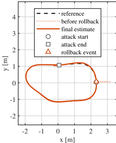
(b) Rollback | RMSE 0.141 m
