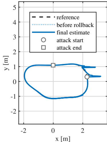
(a) No rollback | RMSE 0.195 m
