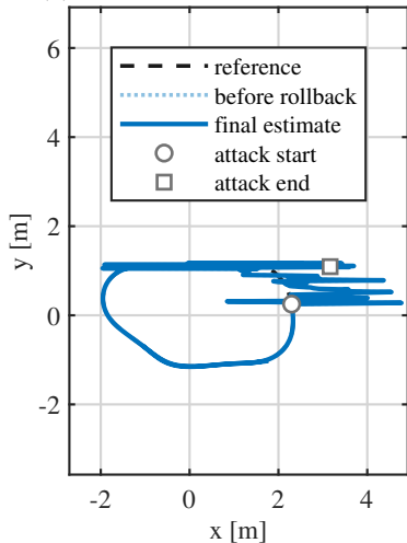
(a) No rollback | RMSE 0.983 m
