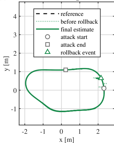
(c) Rollback + anchoring | RMSE 0.042 m
