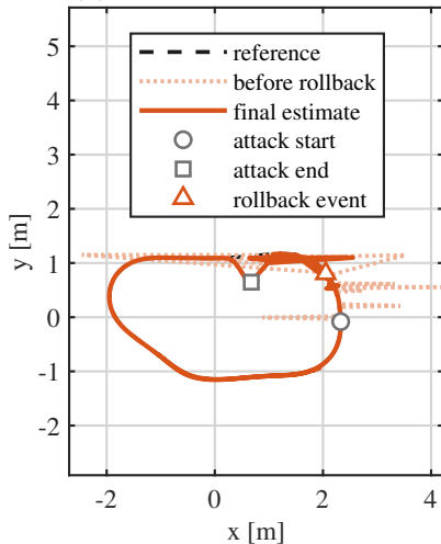
(b) Rollback | RMSE 0.247 m
