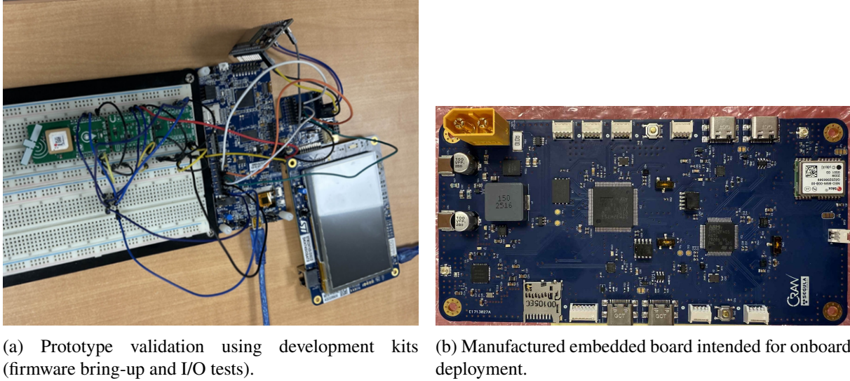
Figure 5.9: Prototype validation and manufactured embedded board.
