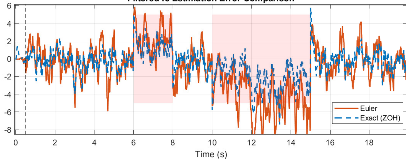
Filtered f^c Estimation Error Comparison
