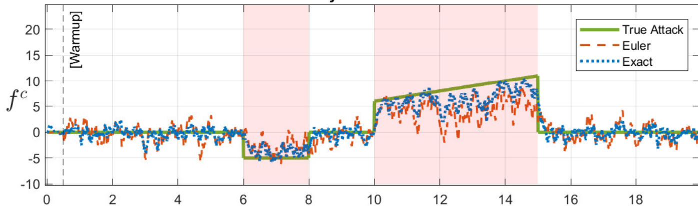
Filtered Cyber-Attack Estimates
